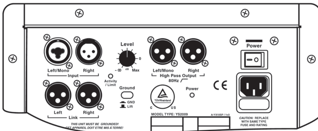
YX10SP Rear Panel
