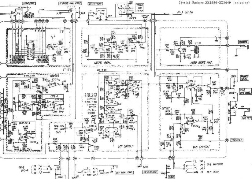
C. Circuit diagram (OP-10B) (Serial Numbers XX2550-XX3049 inclusive)
