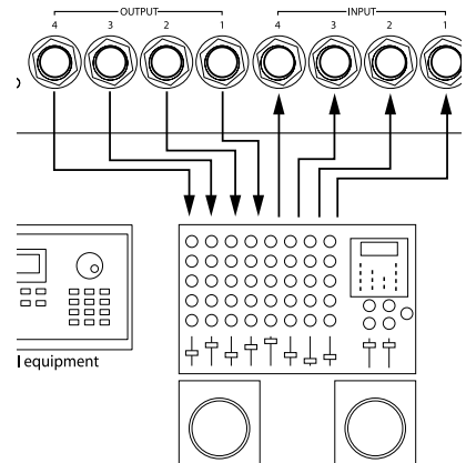
Connecting the G2 to the sound system
