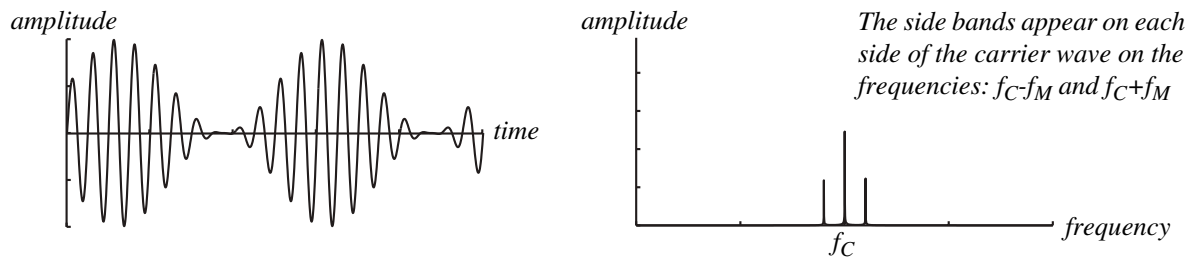
Fig 3. Amplitude Modulation
