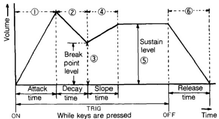
ADBSSR envelope – the diagram right is ripped from the original Poly-800 Owner’s Manual.
