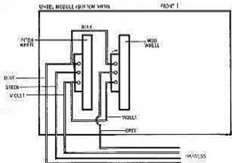
FIGURE 6 - WHEEL MODULE CONNECTIONS
