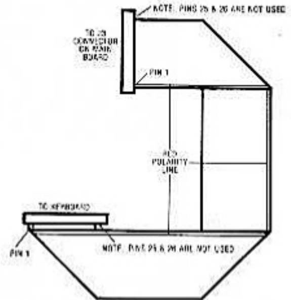
FIGURE 5 - KEYBOARD CABLE
