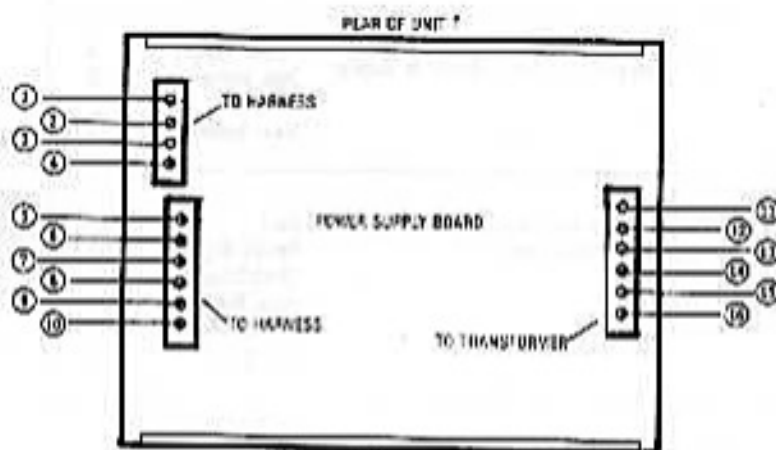
FIGURE 2 - POWER SUPPLY VOLTAGE CHECK POINTS
