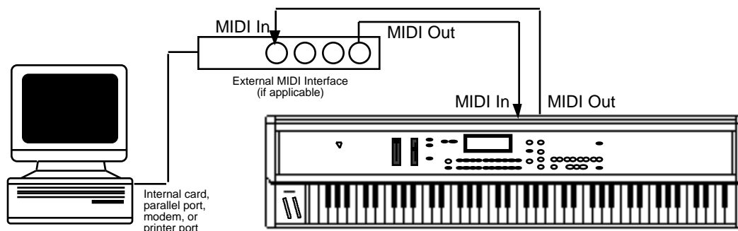
Computer (with MIDI Interface) connected to E-Prime's Keyboard
