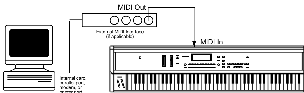
Computer (with MIDI Interface) connected to E-Prime's Keyboard
