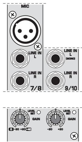
Fig. 2.5: Stereo channel inputs
