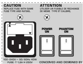
Fig. 2.16: Voltage supply and fuse
