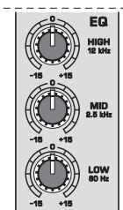
Fig. 2.2: The equalizer of the input channels
