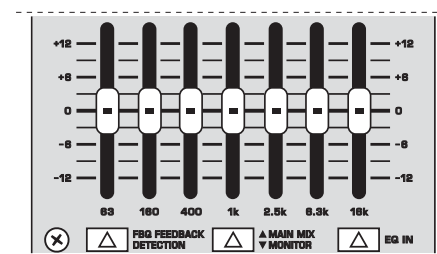
Fig. 2.15: The graphic stereo equalizer
