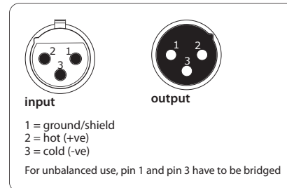
Fig. 4.2: XLR connections
