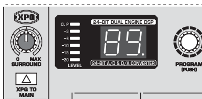
Fig. 3.3: Digital effects module and XPQ surround function control elements
