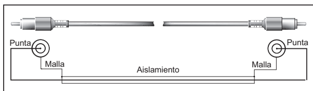
Fig. 5.3: Cable RCA
