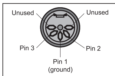
Fig. 9.4: MIDI plug pin assignment
