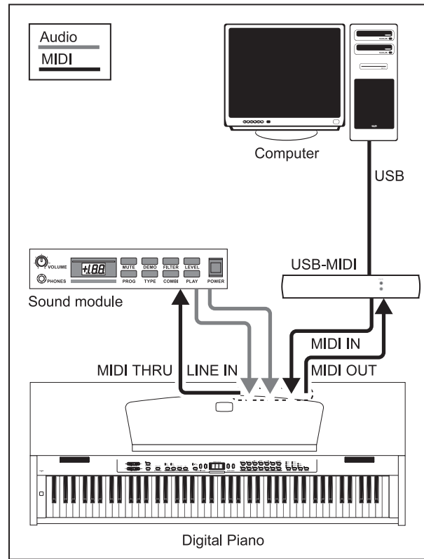
Fig. 6.4: MIDI set-up including a sequencer and external sound module
