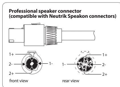
图 1.3 Speakon 插
