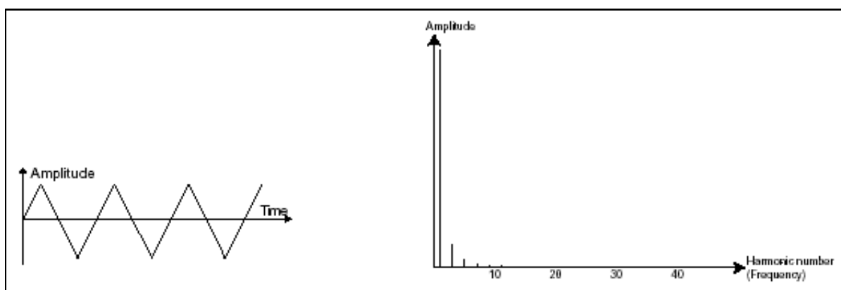
Triangle waveform
