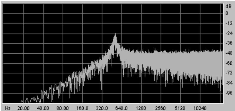
High-pass filter
