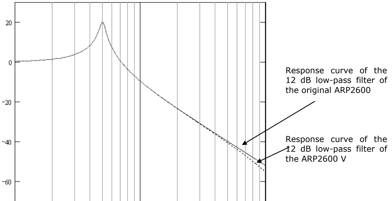
Response curve of the 12 dB low-pass filter of the original ARP2600 and the ARP2600 V
