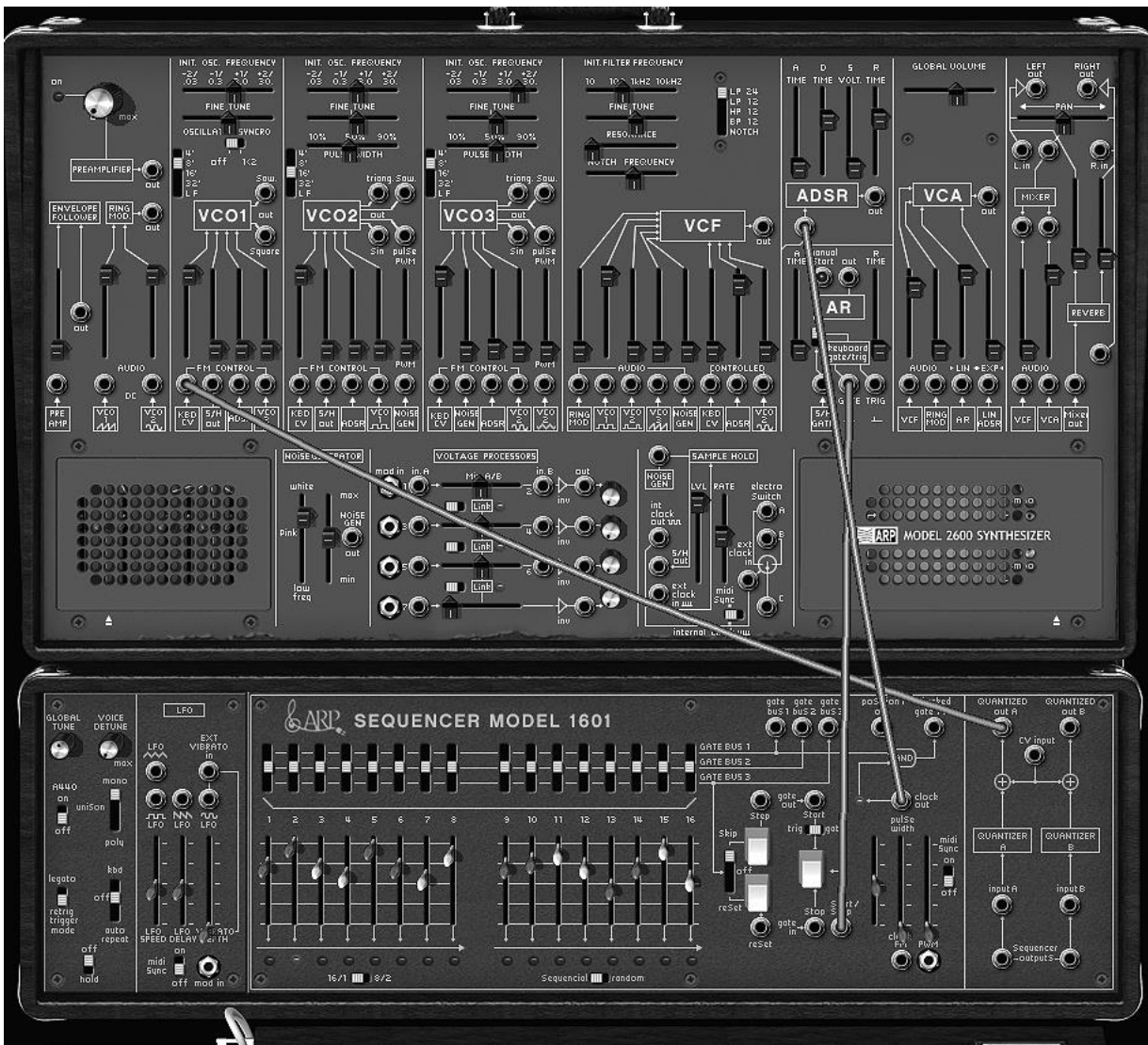
The connections between the sequencer and synthesizer
