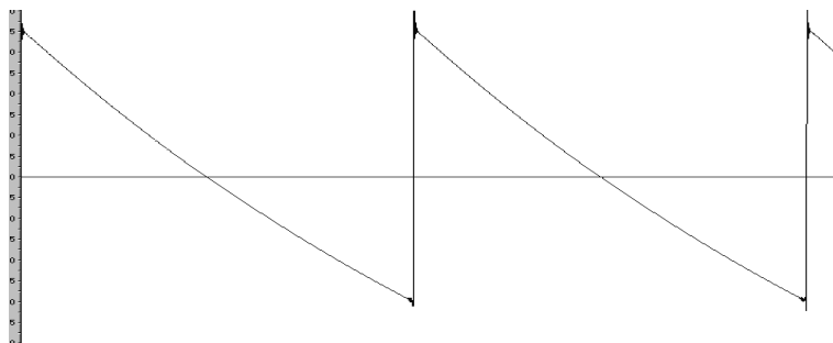
Temporal representation of an ARP2600 V "saw tooth" waveform reproduced by TAE
