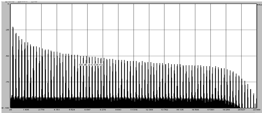
Linear frequency spectrum of the ARP2600 V oscillator made with TAE
