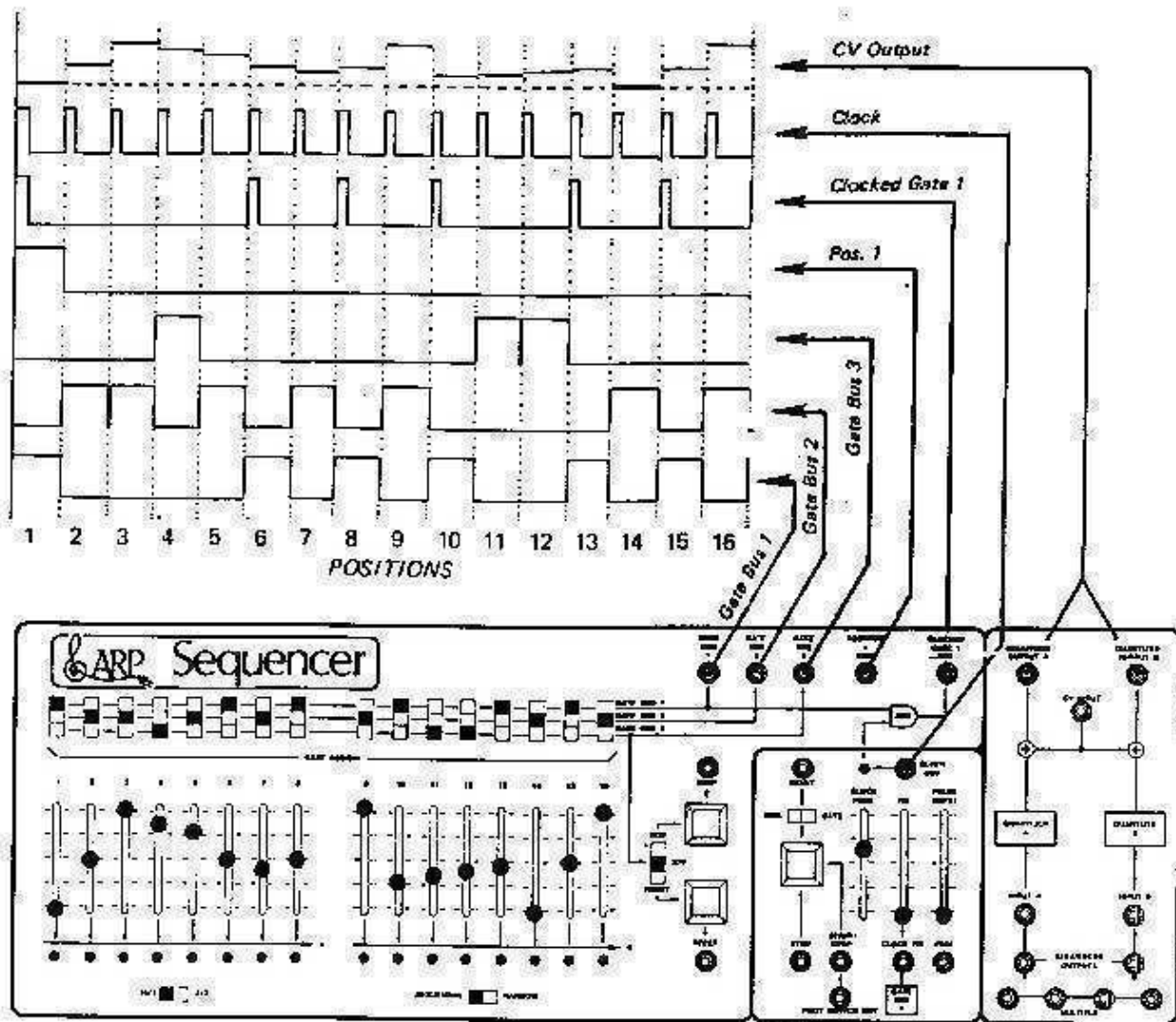
FIG. 2.2 SEQUENCER OUTPUTS
